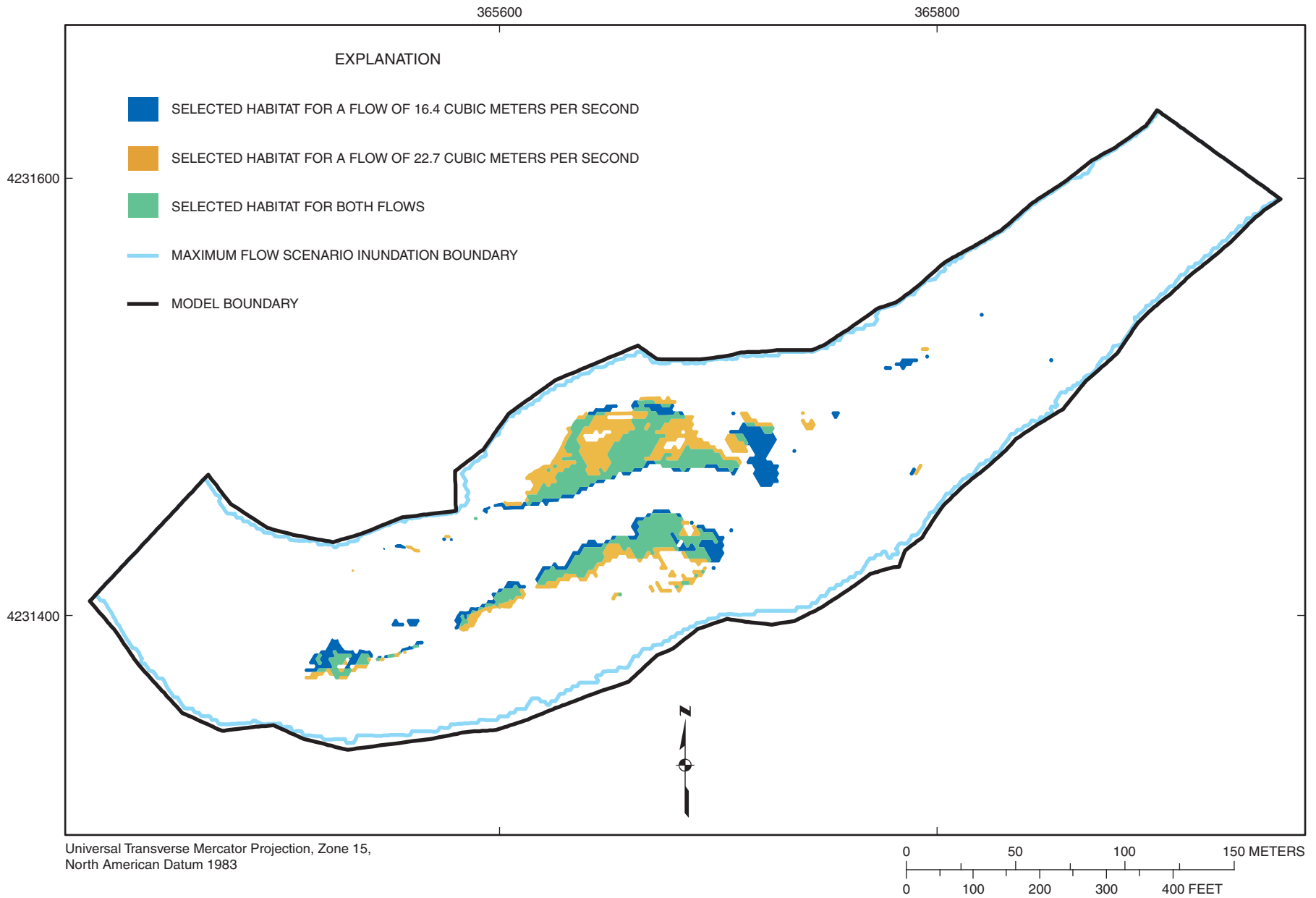
Figure 4-6. Selected habitat area distribution for habitat category 1 (suckermouth minnow) at flows of 16.4 and 22.7 cubic meters per second at Marais des Cygnes River site MDC2.
